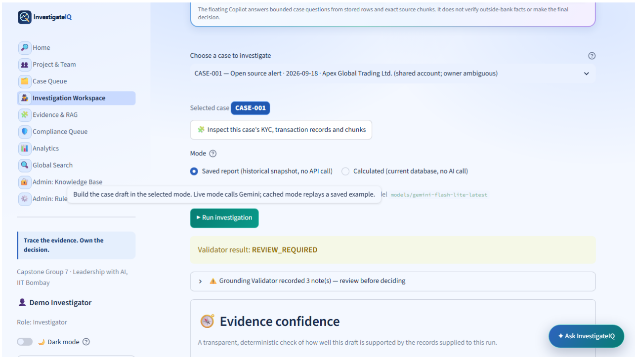
Figure — Workspace report controls and validator result. Run investigation builds or replays a review; it does not record a decision.
